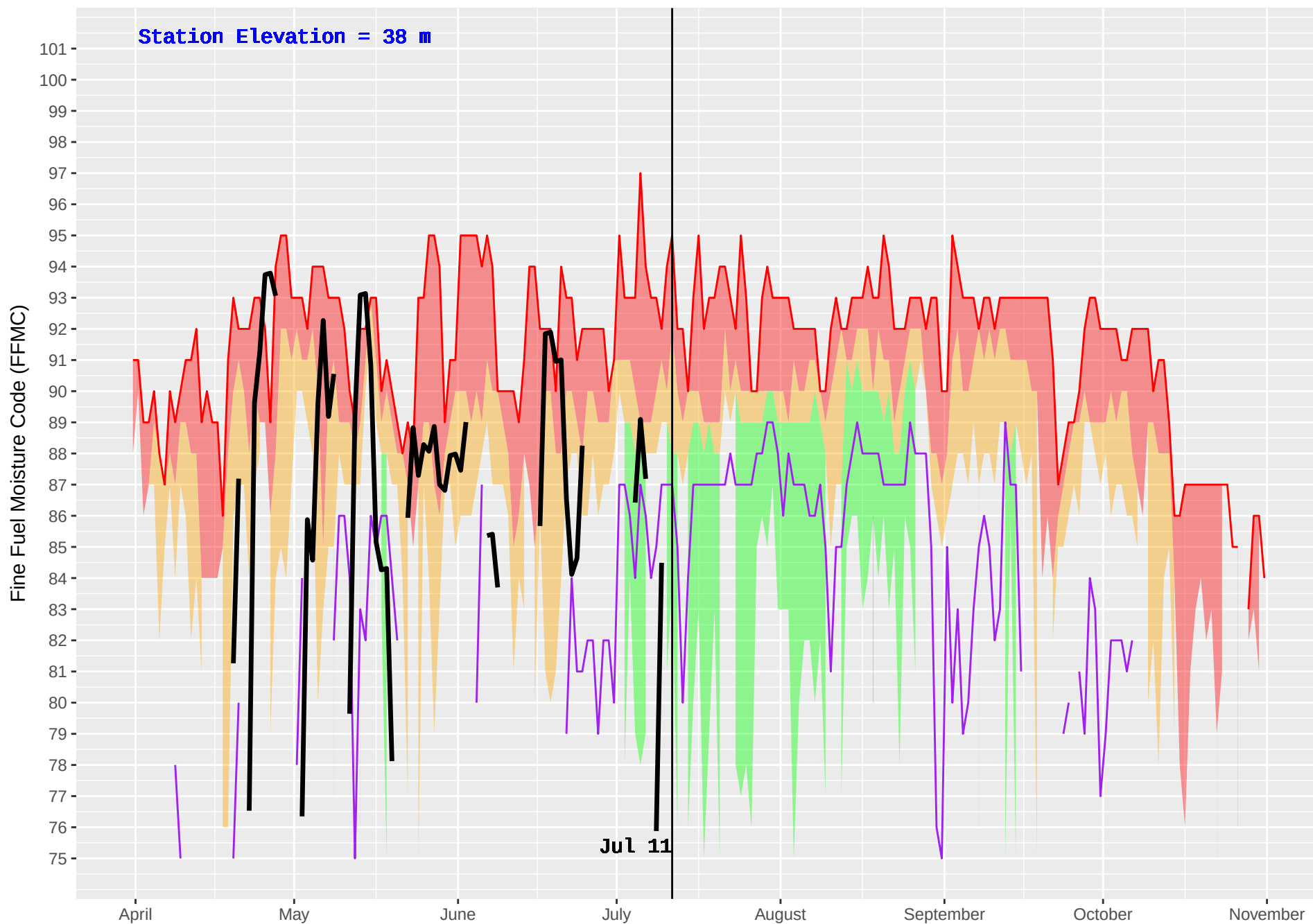
HAIG CAMP (67) : Historical (2002–2016) and Current (2018) Noon Fine Fuel Moisture Code (FFMC)
