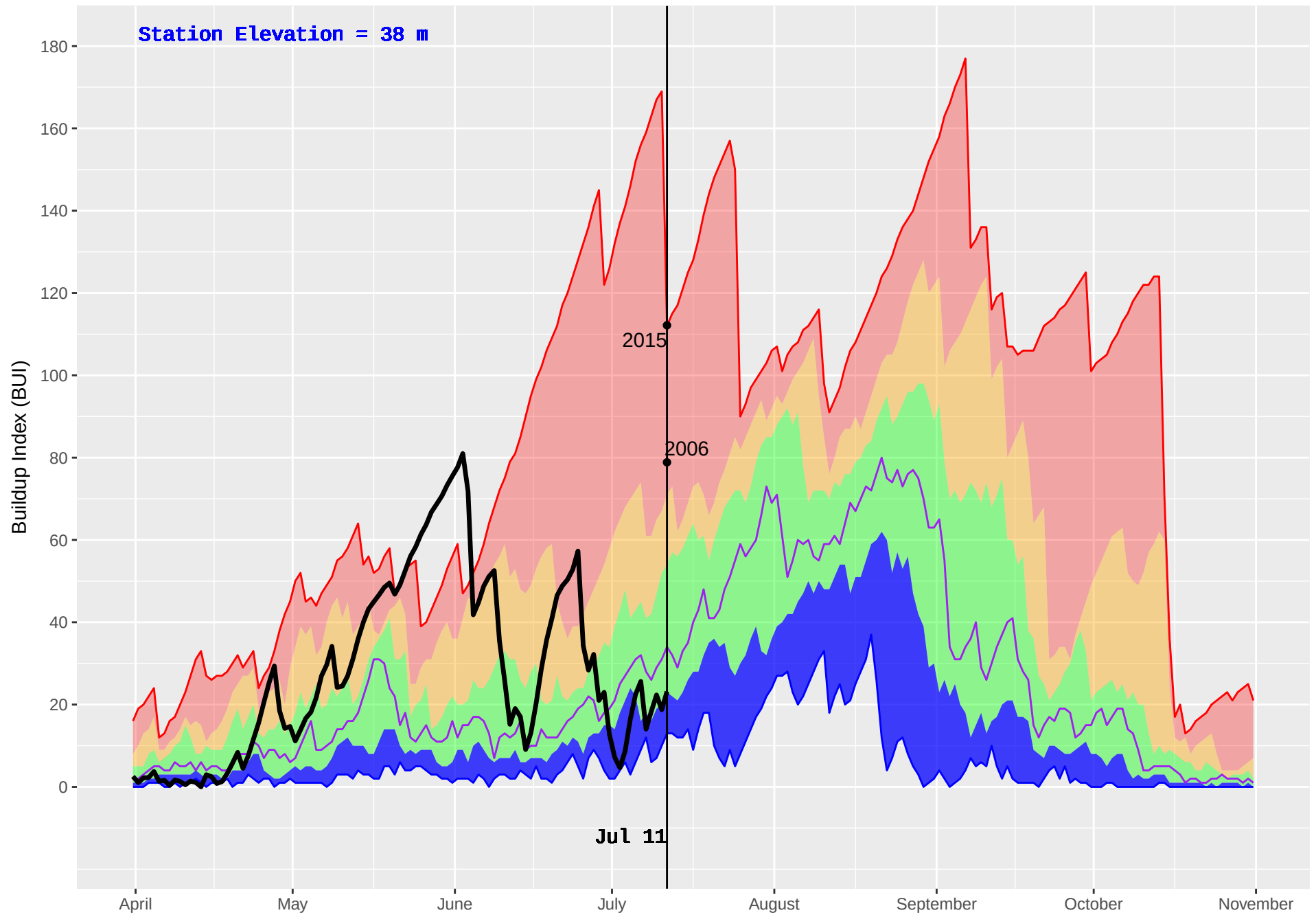
HAIG CAMP (67) : Historical (2002–2016) and Current (2018) Noon Buildup Index (BUI)
